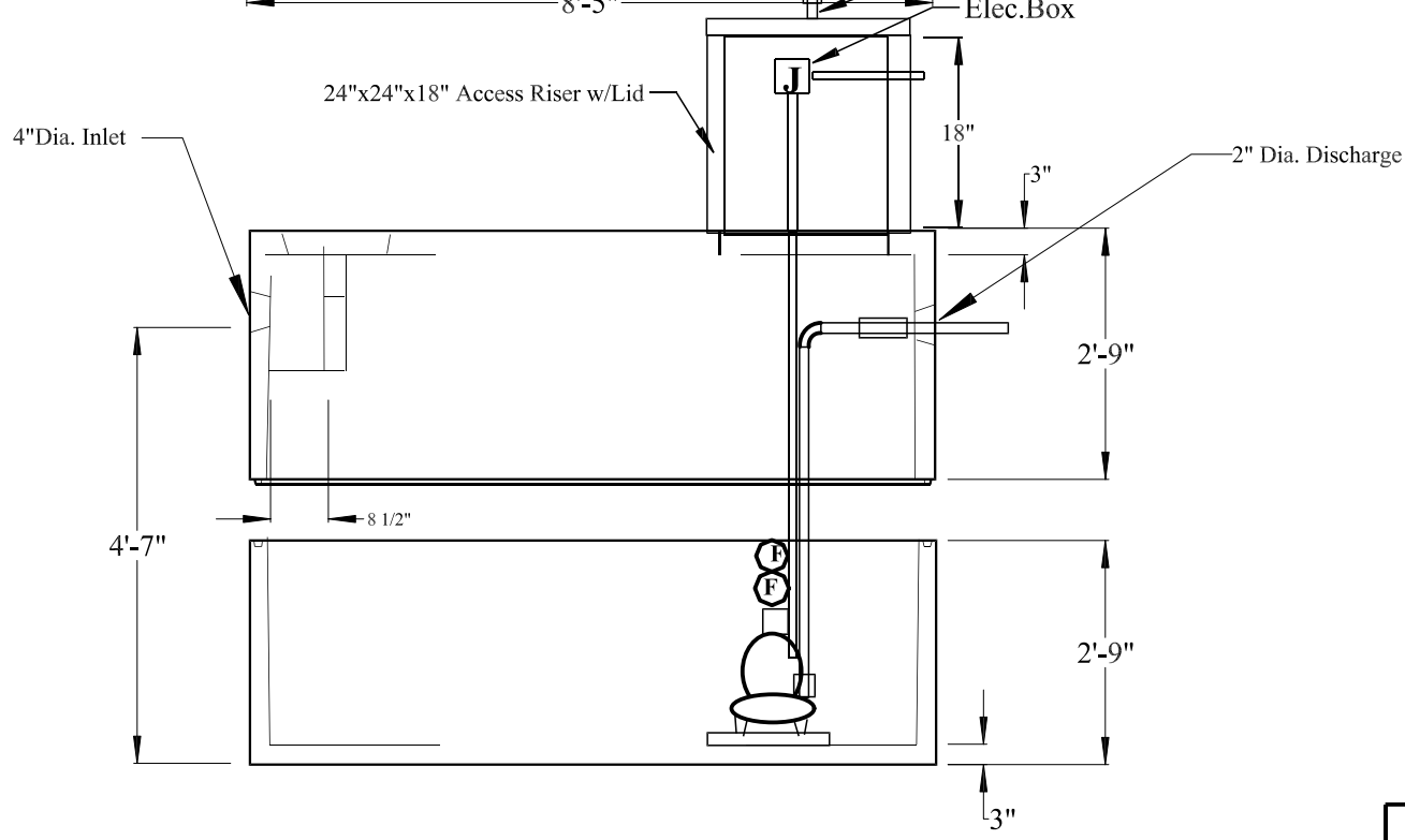
1000 Gallon Lift Station Tank
