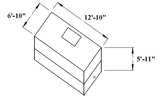
ASSEMBLED TANK
