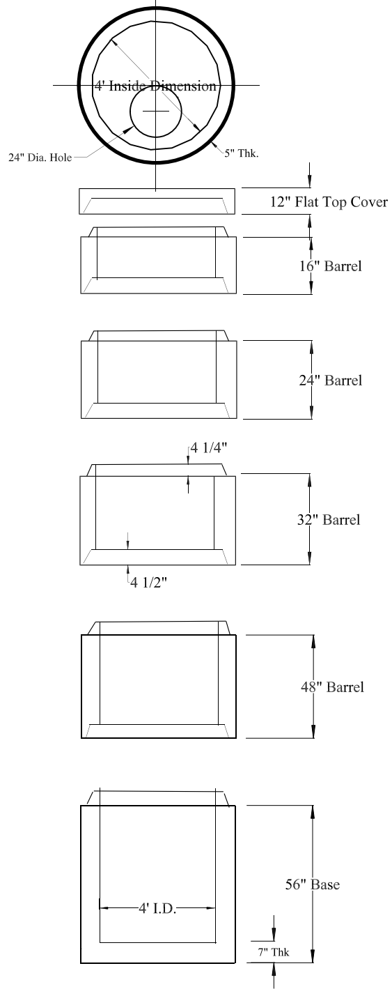
48" I.D. Standard Manhole
