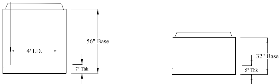
48" I.D. Standard Manhole
